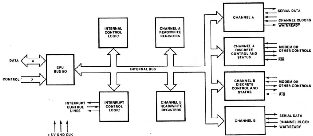
Figure 3. Block Diagram
